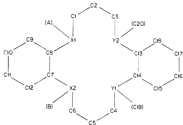
Figure 1. Numbering system used in presentation and discussion of crystallographic results. All structures were numbered so that the distance X1...Y1 is greater than the distance X2...Y2. Coordinates have been presented so that the torsion angle C2–C1–X1–C8 is negative (see Figures 2 and 4). Identity of heteroatoms: 3A and 3B , X1 = X2 = Y1 = Y2 = P(Ph); 4 , X1 = X2 = P(Ph), Y1 = Y2 = S; 5 , X1 = X2 = P(Ph), Y1 = Y2 = N(Me); 6 , X1 = X2 = P(Ph), Y1 = Y2 = O.
