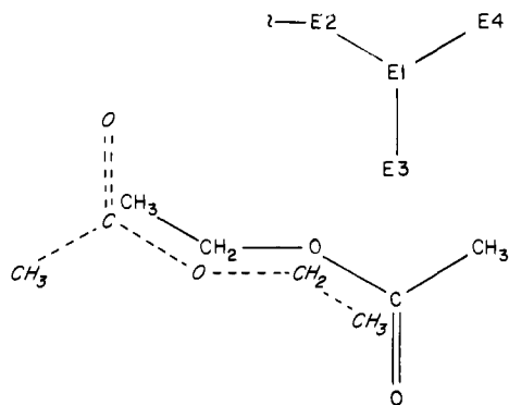
Figure 5. The disorder in the ethyl acetate solvent of crystallization in the crystal structure of 6 . The inversion center at (0, 0, 1/2) is midway between the methylene carbon and the alkoxy oxygen.
